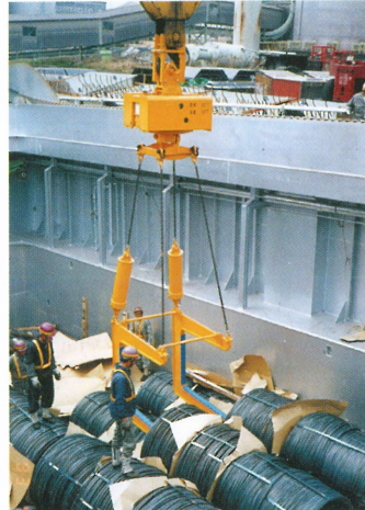
Rotating hook / wire hook
