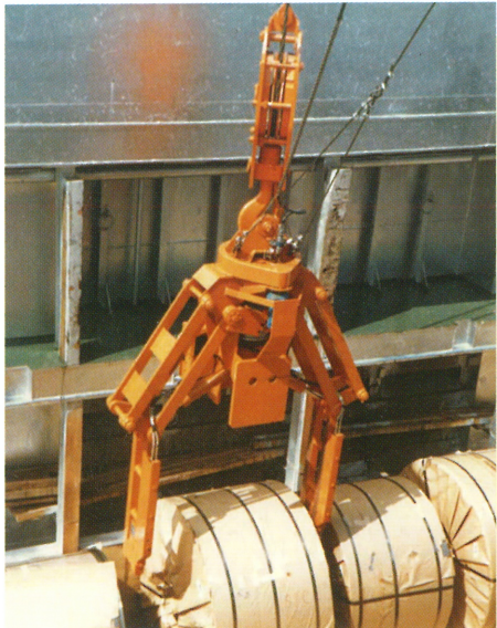
20t vertical coil lifter for shore handling
